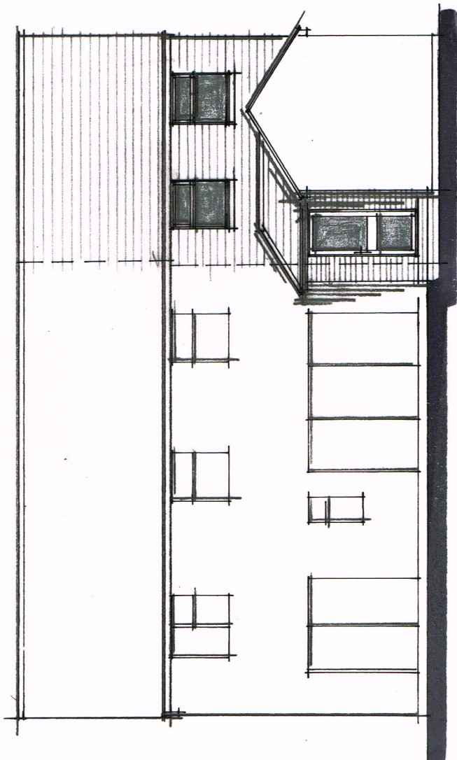
REAR (s) ELEVATION 1:100 @ A3
