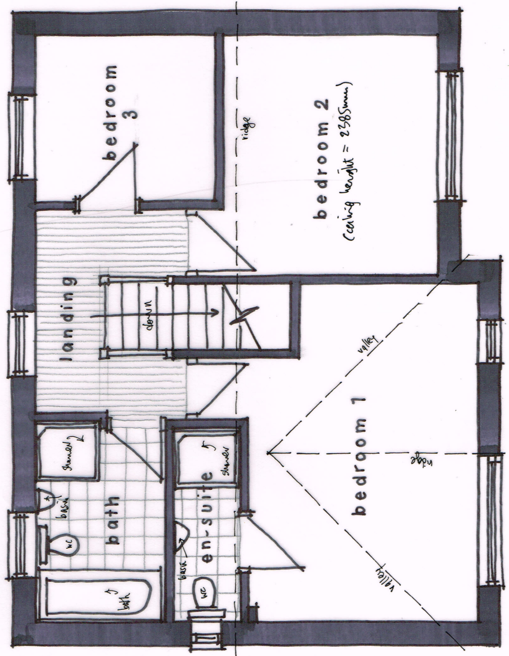
1st FLOOR PLAN 1:50
