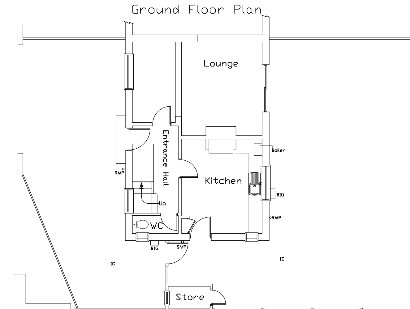
EXISTING FLOOR PLANS 1:100
