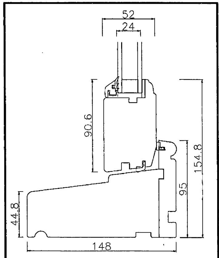
Sill
