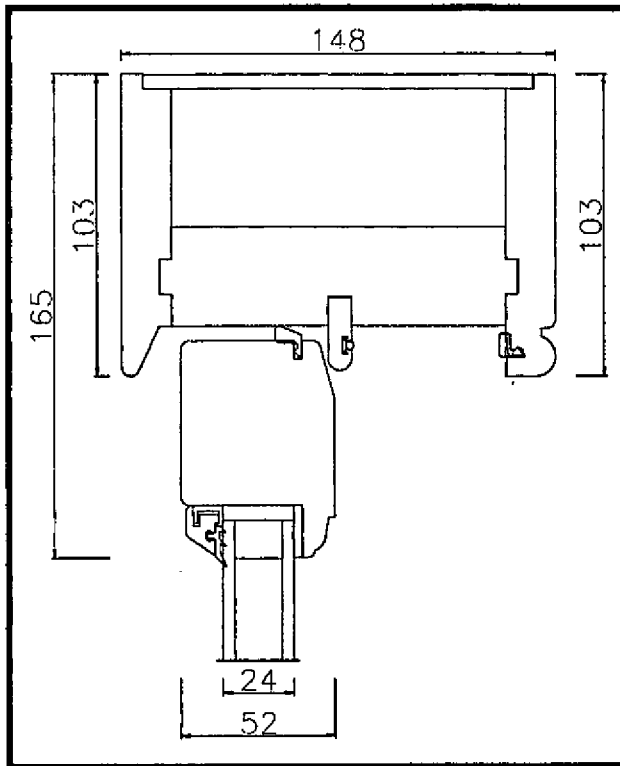
Head
