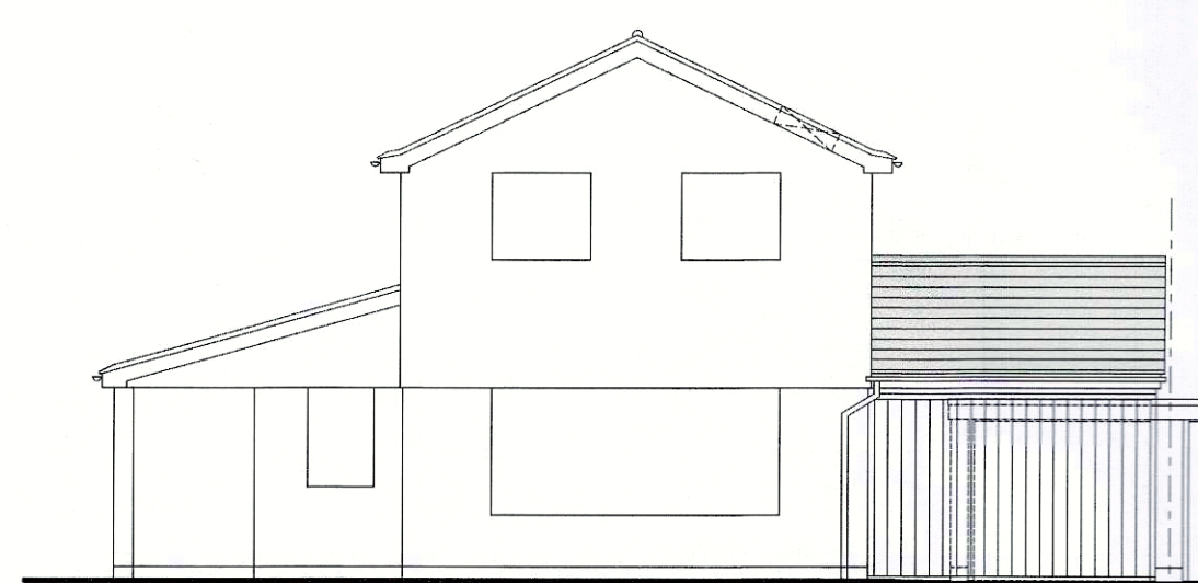
EAST ELEVATION 1/100
