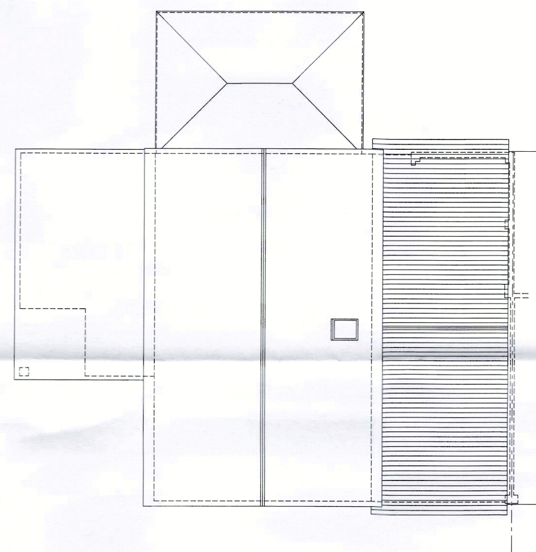
ROOF PLAN 1/100
