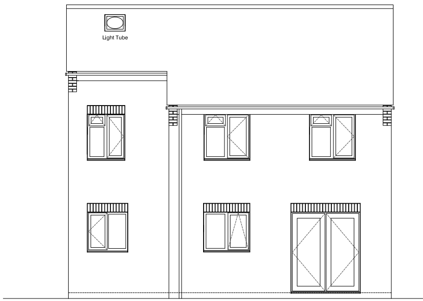
EAST ELEVATION
