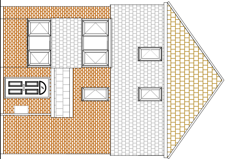
NORTH ELEVATION EXISTING
