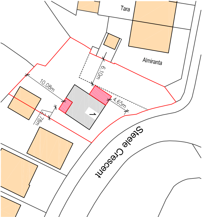
Site Plan 0m 5m 10m 15m 20m 1:500 Scale bar
