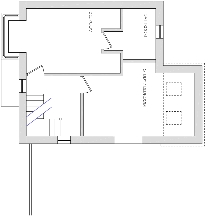
FIRST FLOOR PLAN EXISTING
