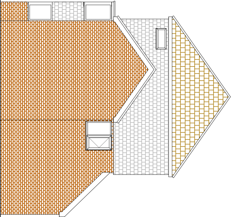
NORTH ELEVATION PROPOSED
