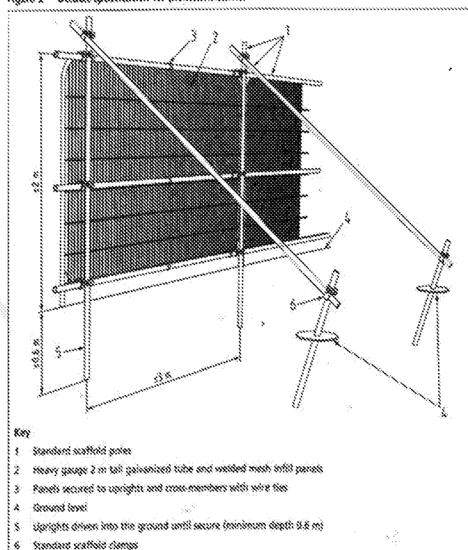
Figure 2 Default specification for protection barrier
