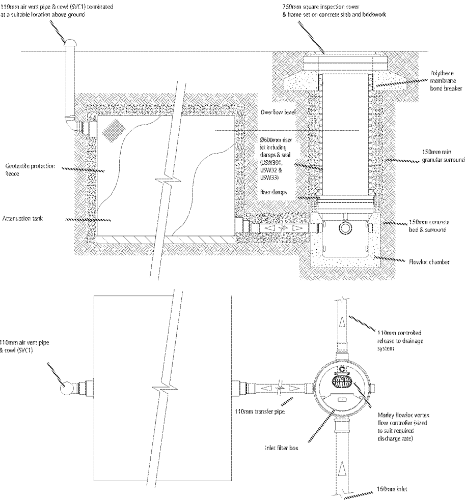
Offline attenuation tank with air vent and Flowloc vortex flow control unit
