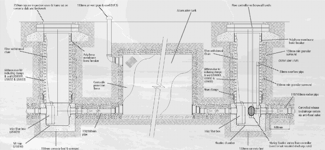
Level invert attenuation tank with air vent, inlet filter and Flowloc vortex flow control unit
