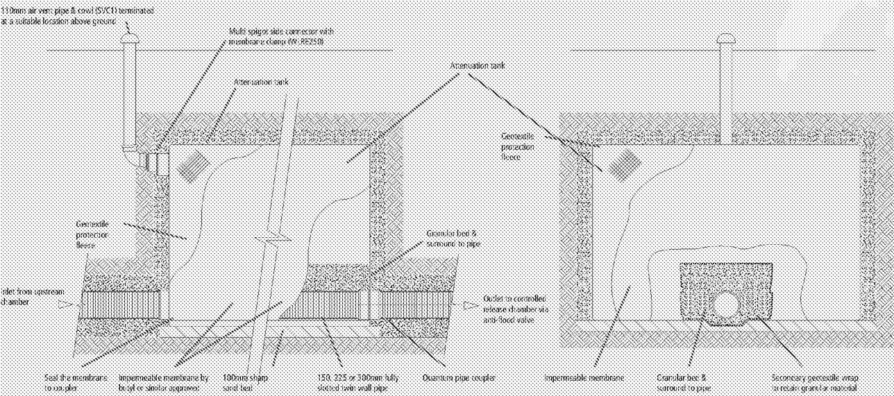
Level invert to attenuation tank using Marley Quantum fully slotted twin wall pipe and air vent
