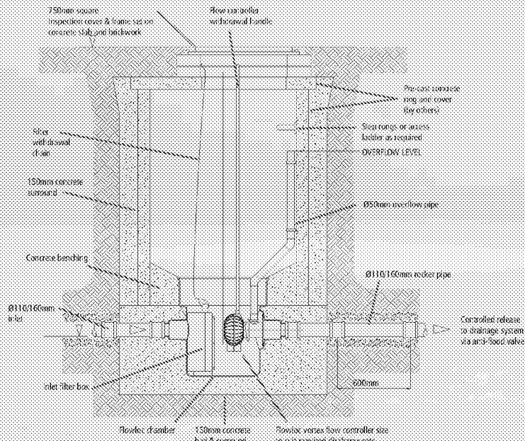
Marley Flowloc chamber with concrete riser and Flowloc vortex flow control unit
