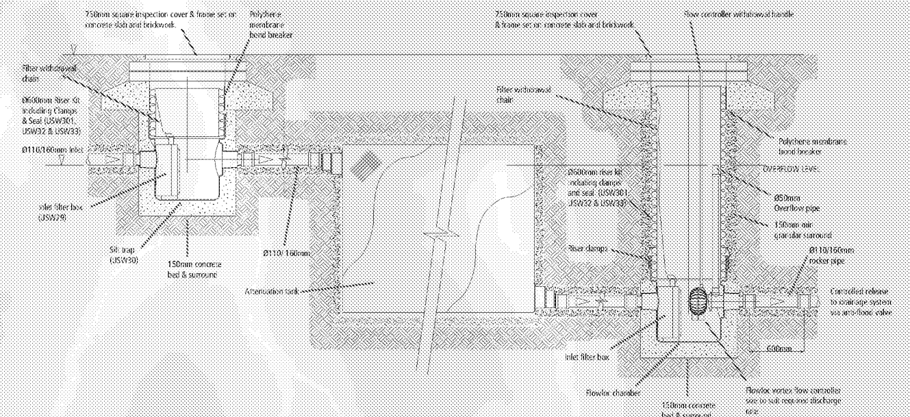
Level invert attenuation tank with air vent, inlet filter and Flowloc vortex flow control unit
