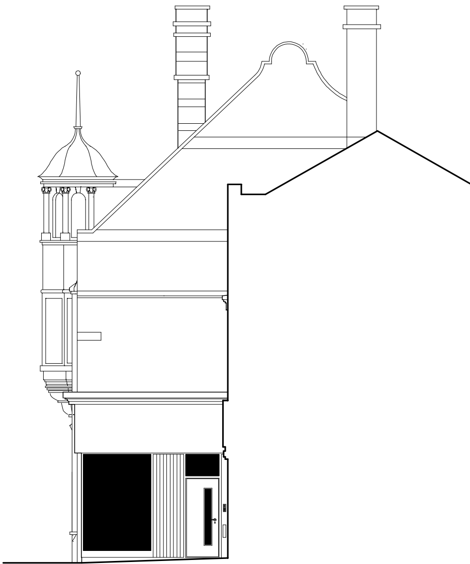
West Elevation as proposed
