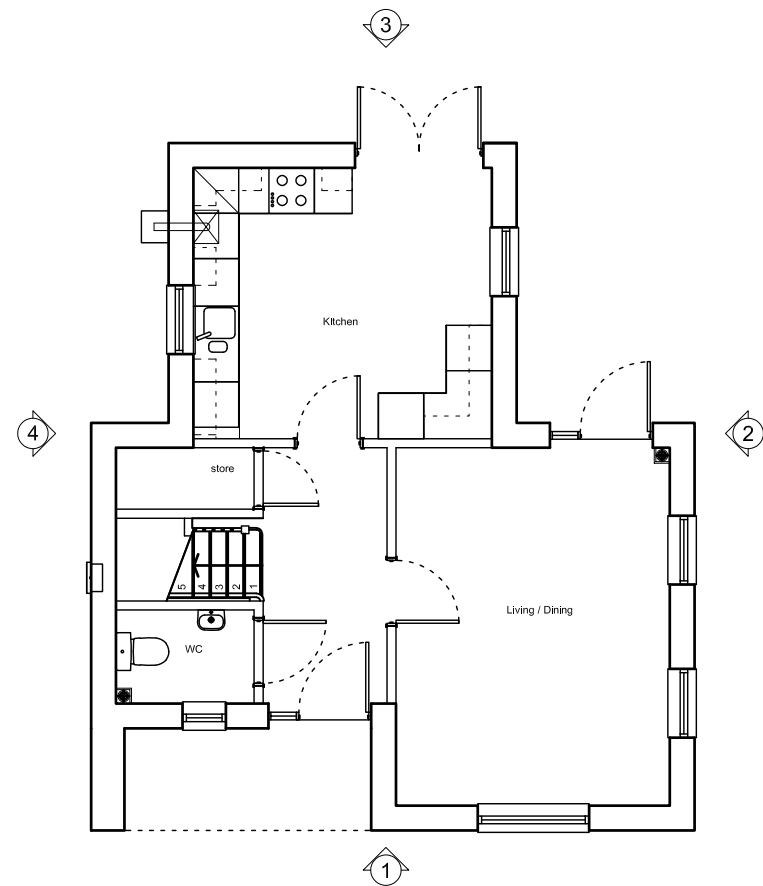
01 Ground Floor Plan 2140 Scale: 1:100
