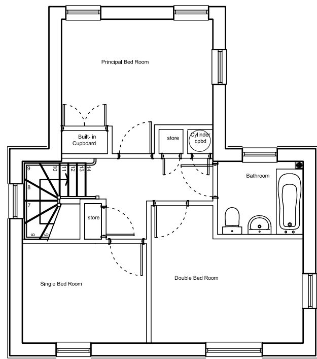
02 First Floor Plan 2140 Scale: 1:100
