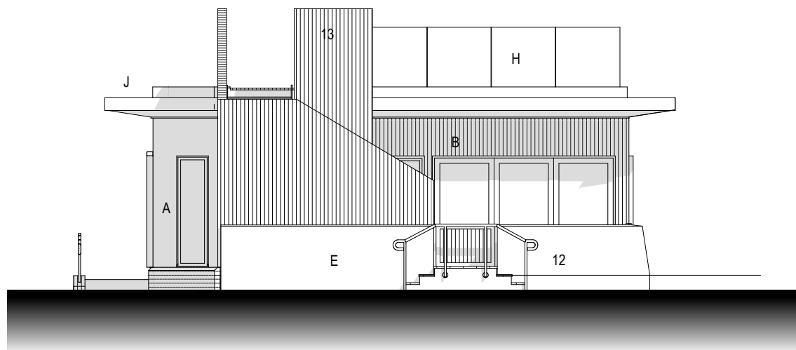
West Elevation Proposed
