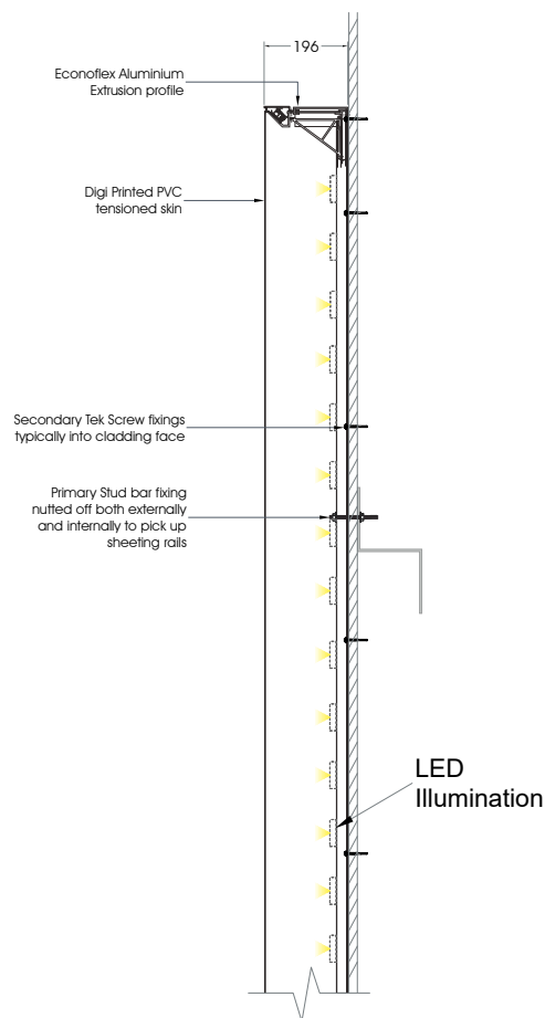
ECONOFLEX BOX TYPICAL SECTION
