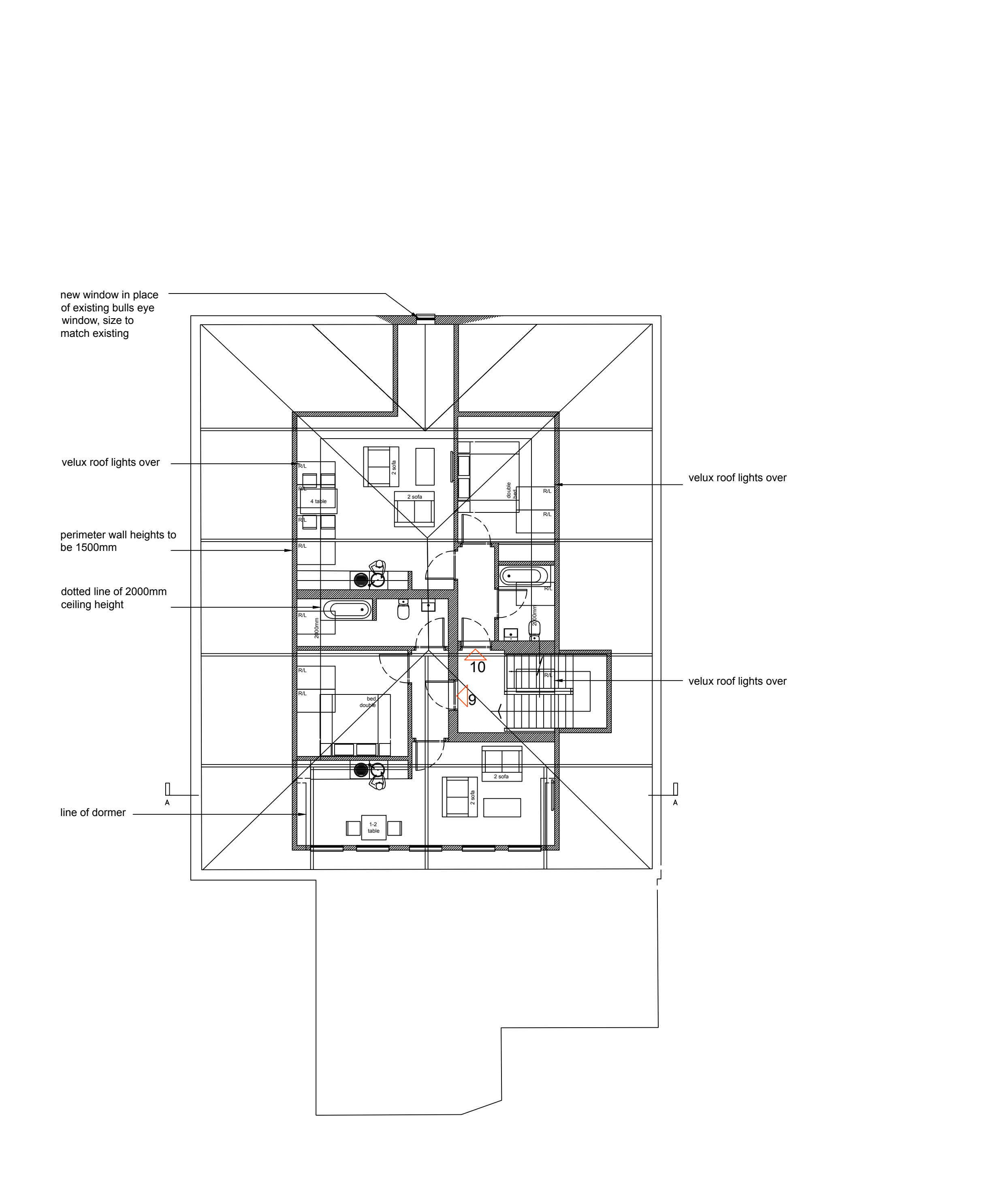
Loft Level Plan
