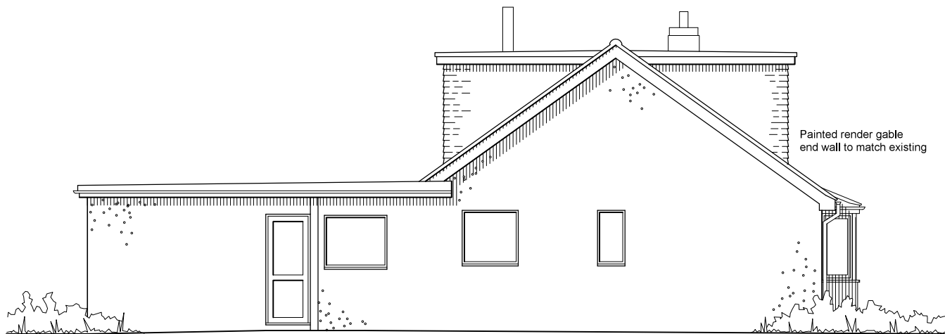
East Elevation
