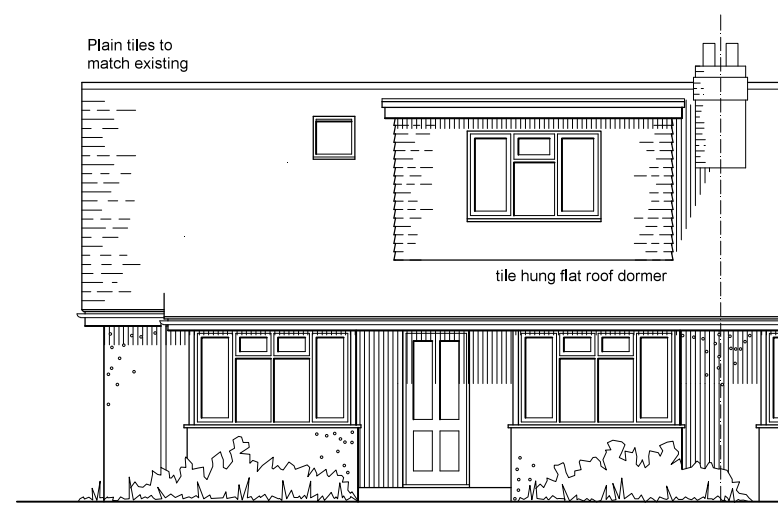
North Elevation
