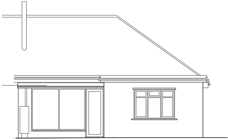
South Elevation
