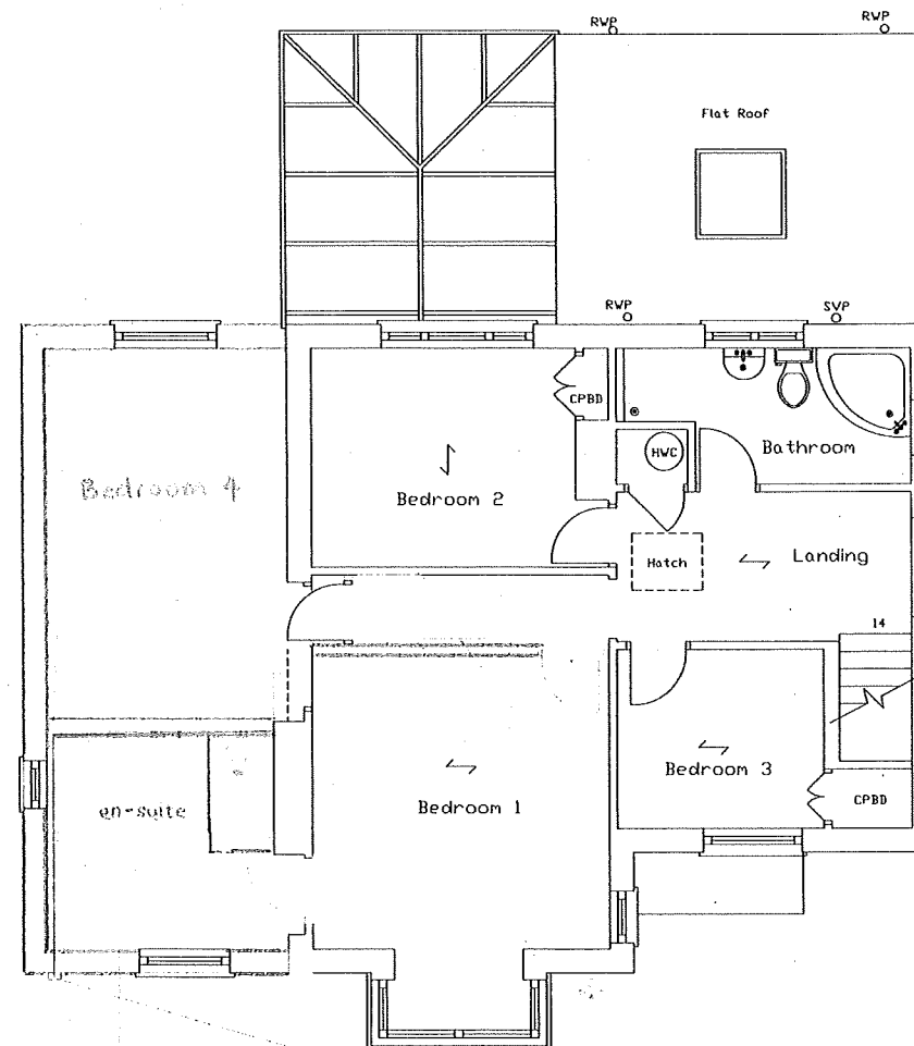
EXISTING FLOOR PLANS 1:100
