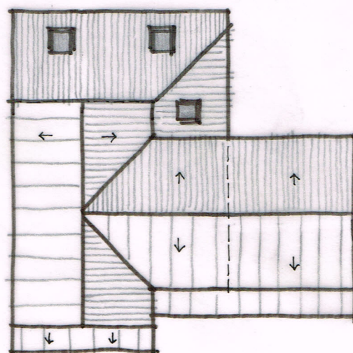
ROOF PLAN 1:200
