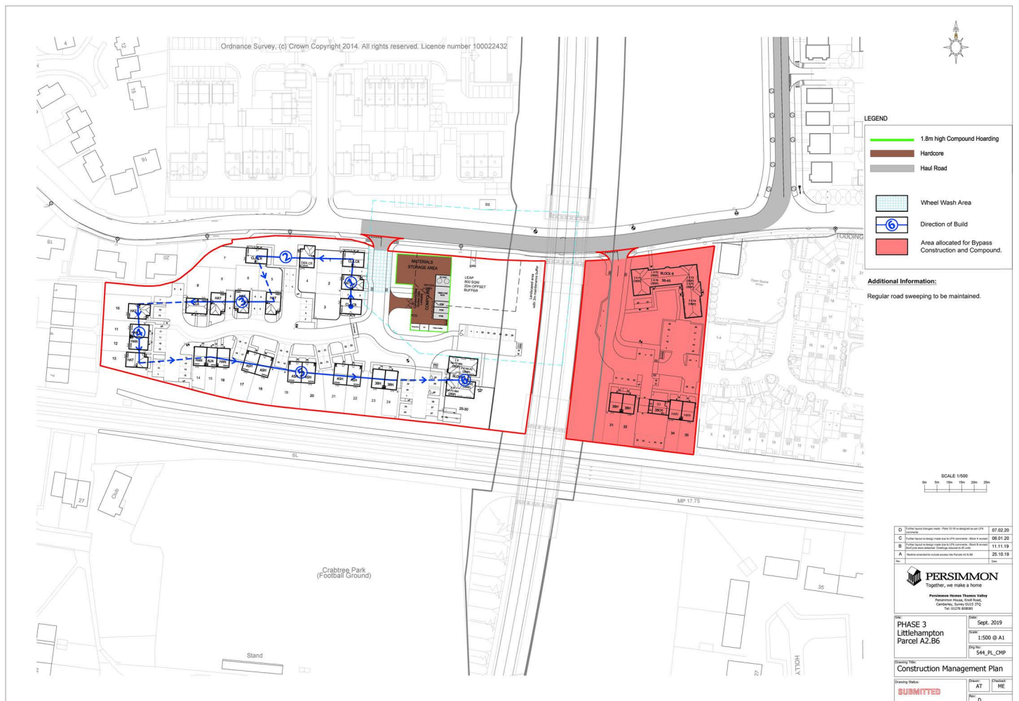
Image 1: Construction Compound Layout
