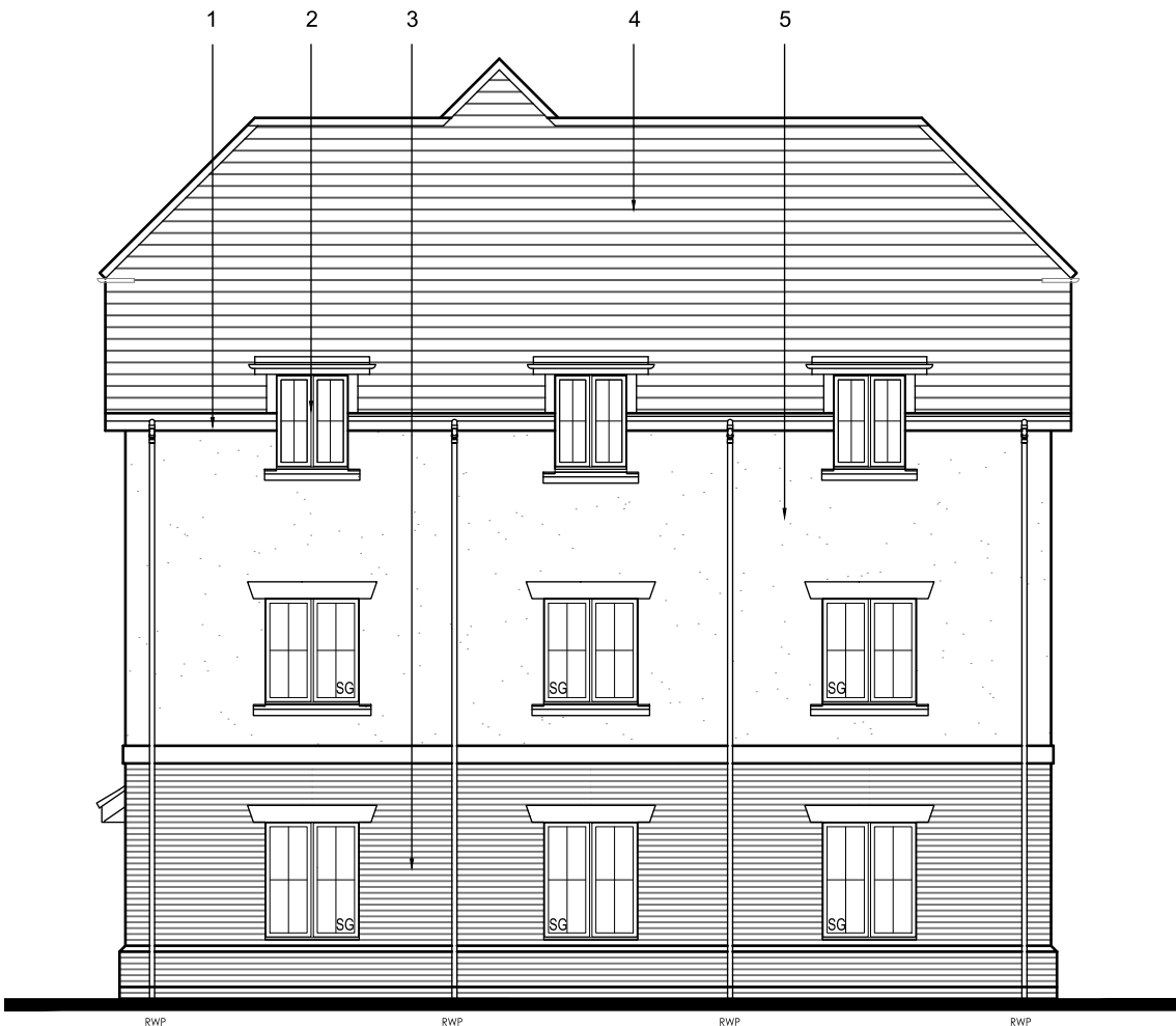
Side Elevation
