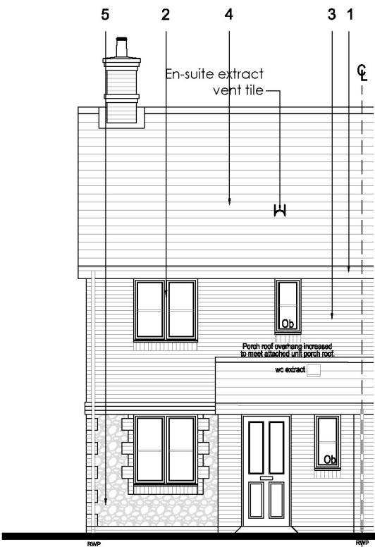
Front Elevation Plot 13H only
