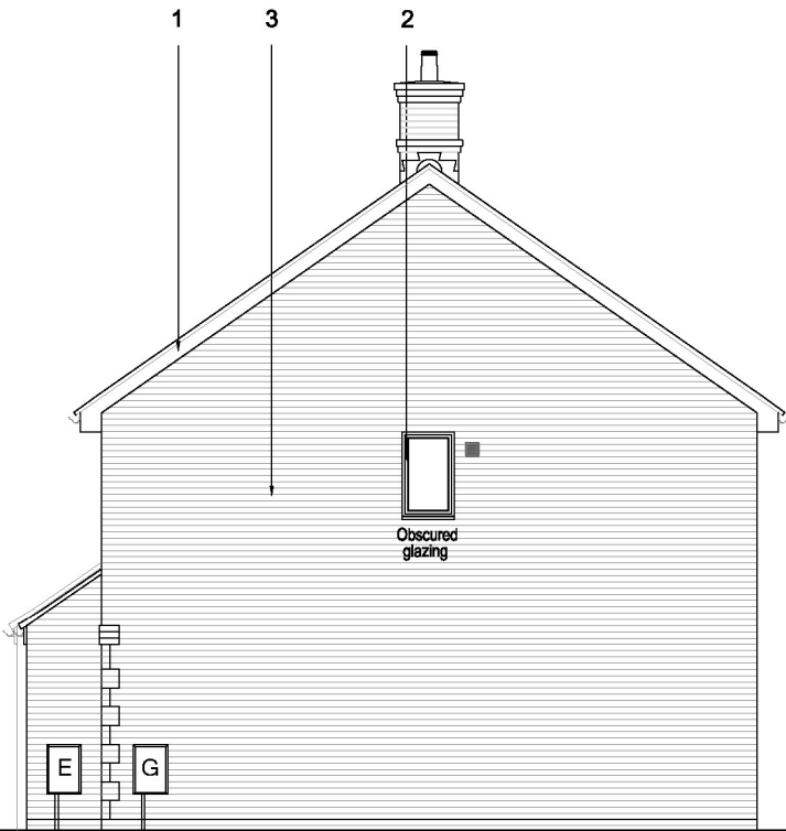
Side Elevation Plots 11 & 16H only
