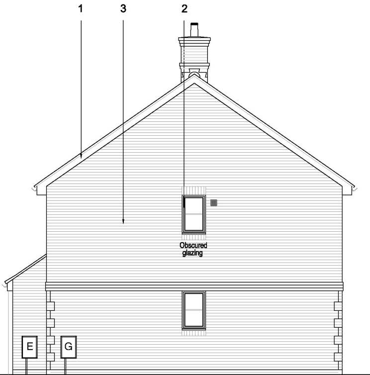
Side Elevation Plot 15 only
