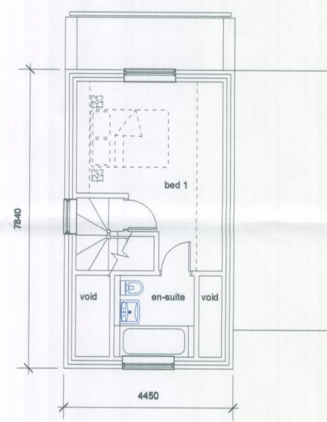
second floor 1:100
