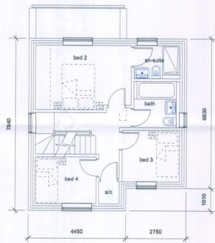
first floor 1:100
