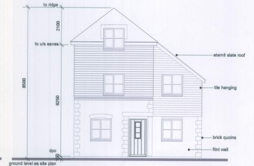
west (front) elevation 1:100
