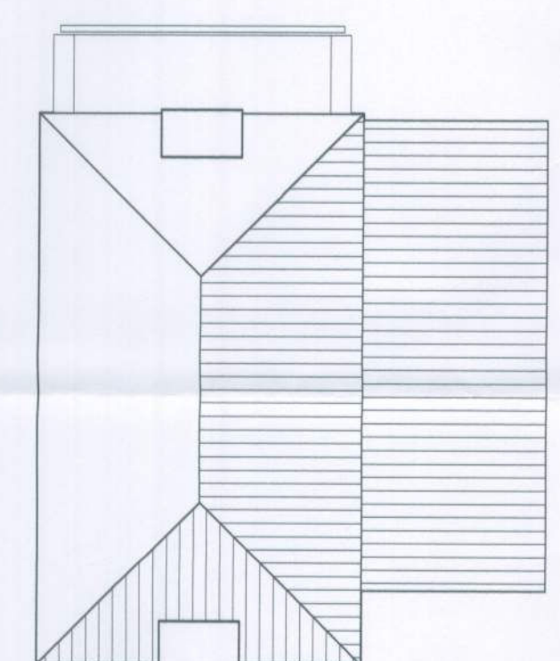
roof plan 1:100
