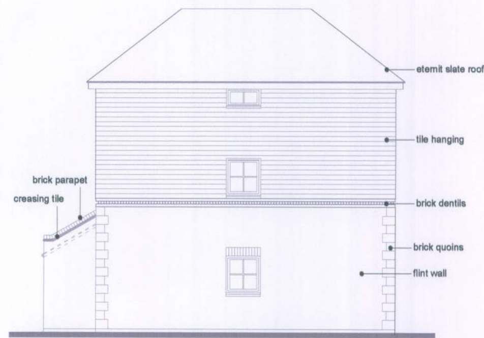
north (side) elevation 1:100
