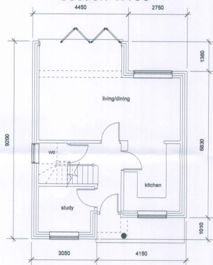
ground floor 1:100
