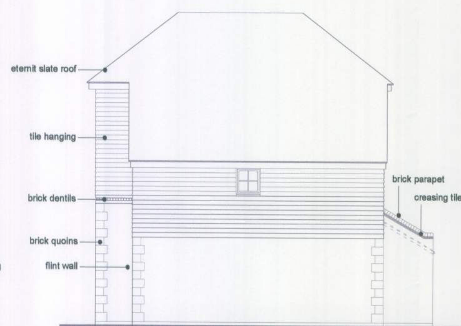
south (side) elevation 1:100
