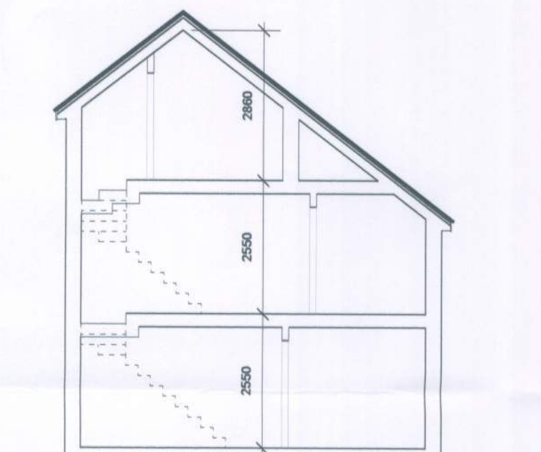
section 1:100
