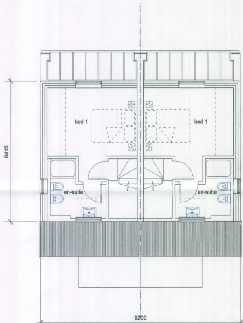
second floor
