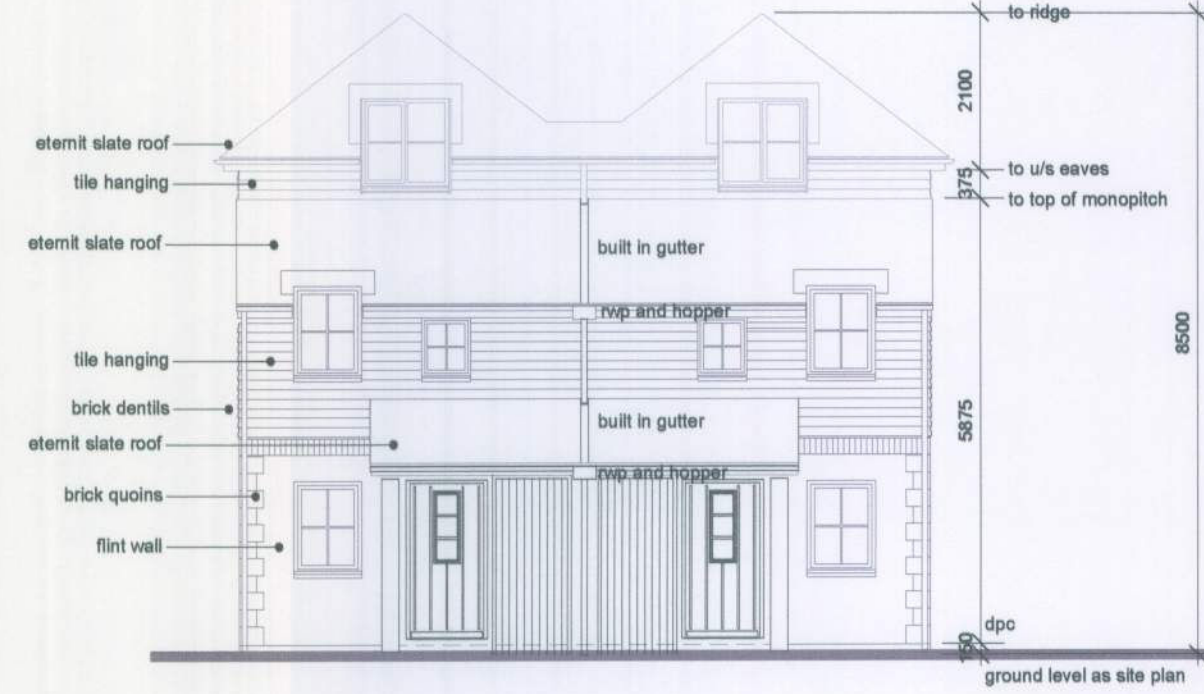
east (front) elevation 1:100
