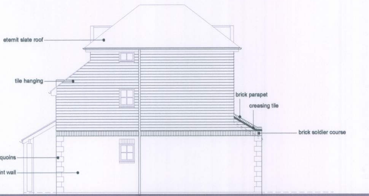
north (side) elevation 1:100 (south handed)
