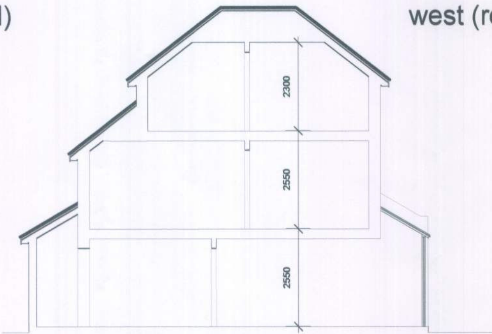
section 1:100
