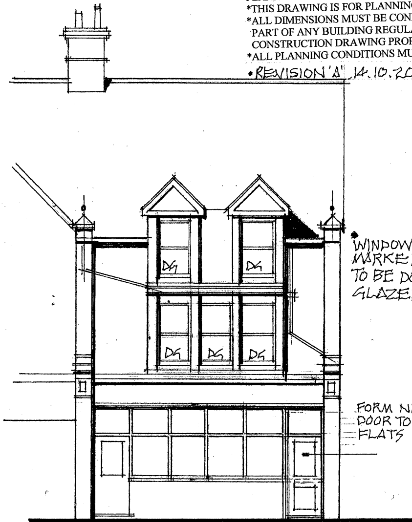
FRONT ELEVATION PROPOSED/BEACH ROAD
