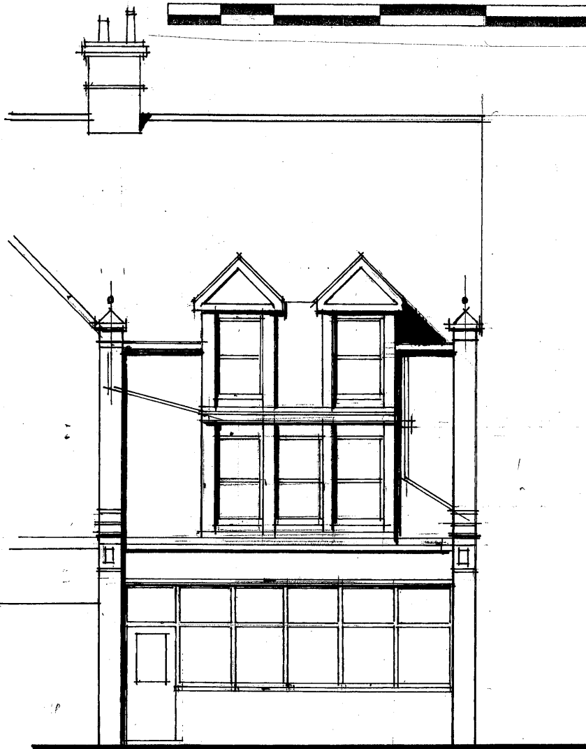
FRONT ELEVATION EXISTING/BEACH RD.
