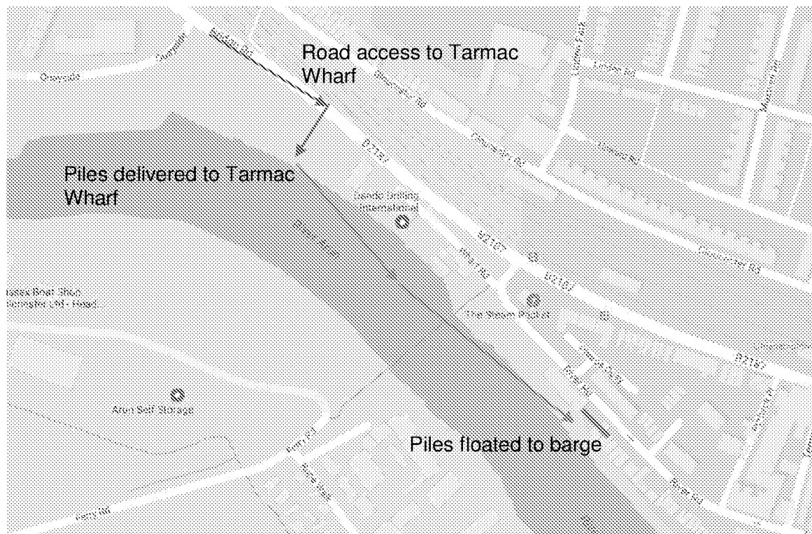
Figure 2 - Sheet Pile Access Route
