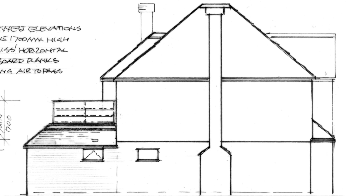
PROP. EAST ELEVATION 1:100
