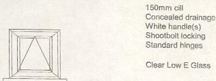
White Casement window - WC 2nd floor - 400mm W x 500mm H
