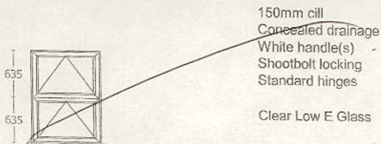
White Casement Window - 2nd floor front - 800mm W x 1300mm H - 2 pan
