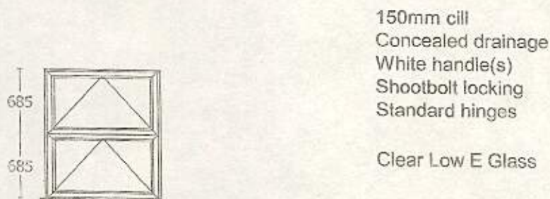
White Casement Window - 2nd floor rear - 1000mm W x 1400mm H
