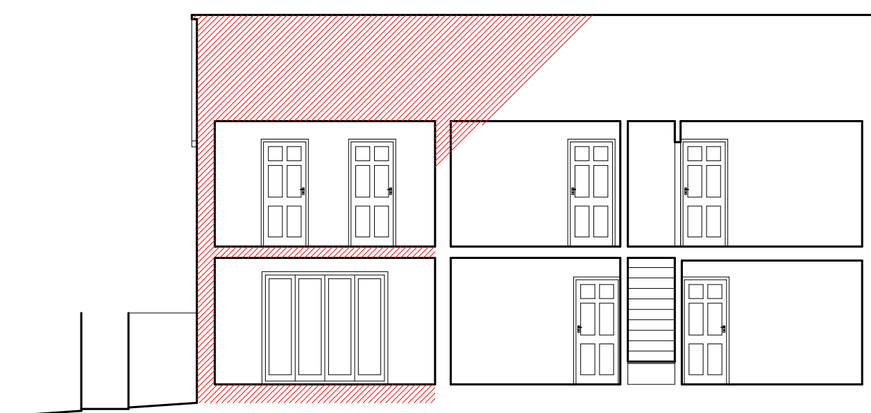
SECTION looking North as proposed
