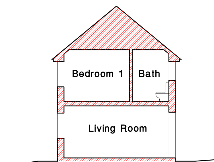
SECTION looking West as proposed
