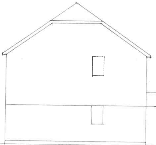
east elevation
