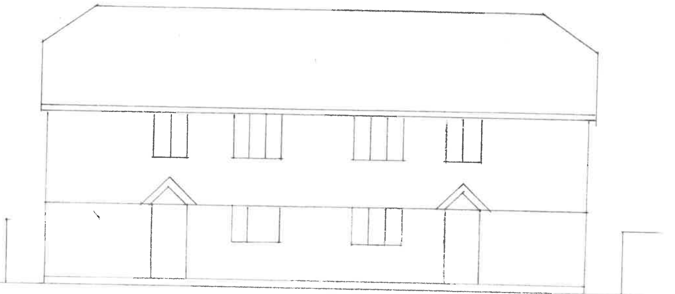
front elevation
