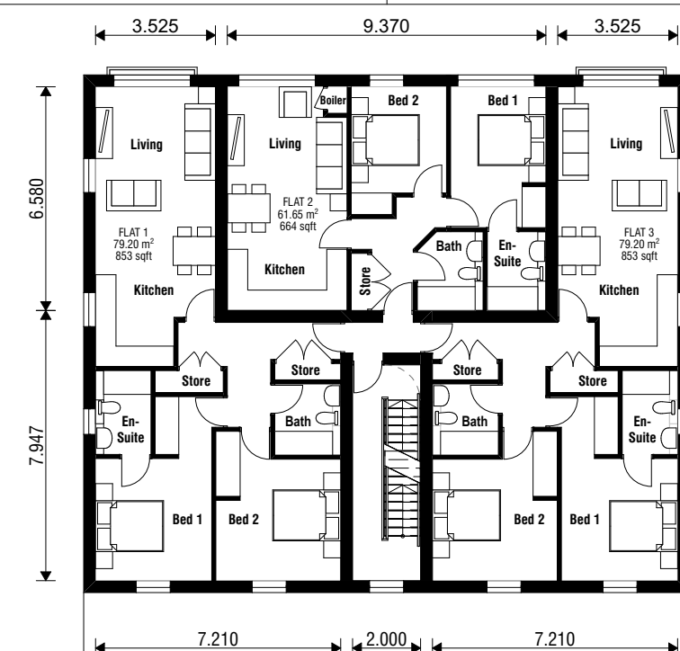
0. Proposed First Floor 1:200
