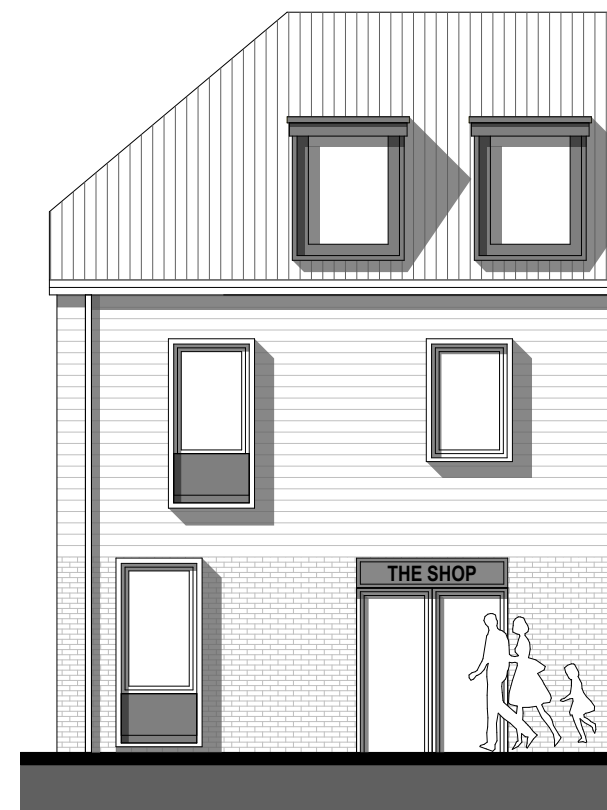
Proposed Front Elevation Extract 1:100
