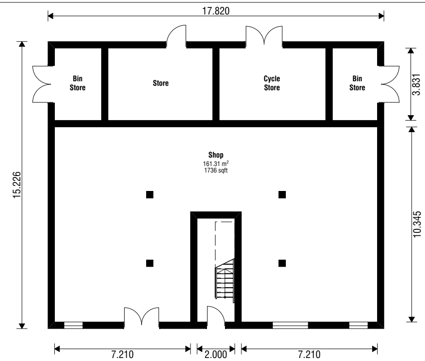
0. Proposed Ground Floor 1:200
