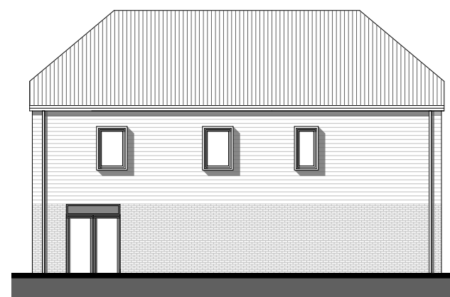
Proposed Typical Side Elevation 1:200
