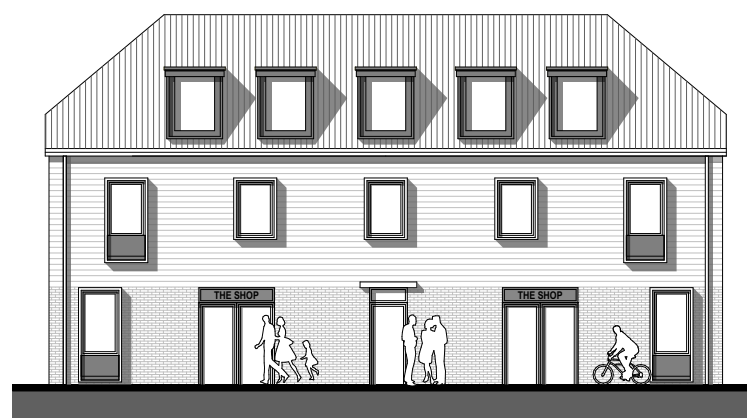
Proposed Front Elevation 1:200
