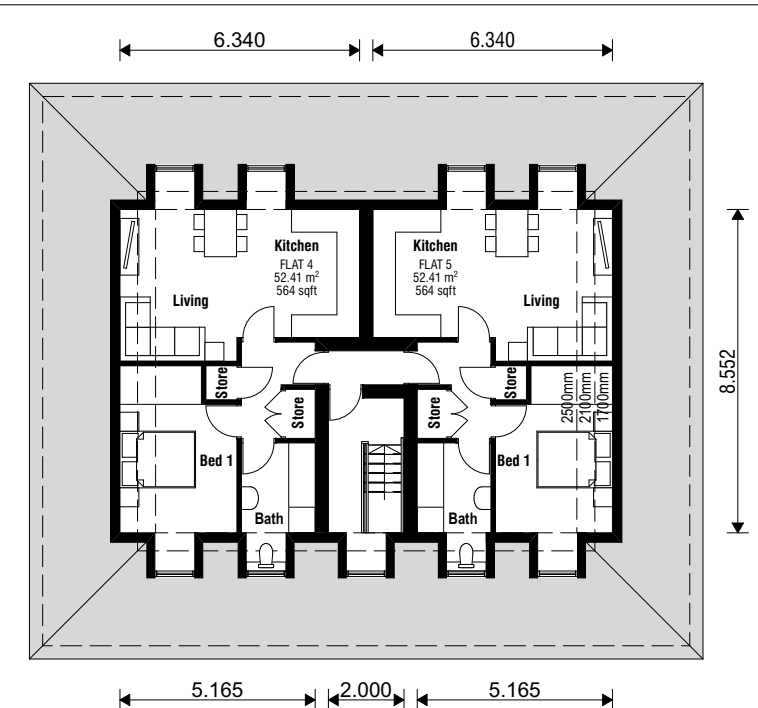
0. Proposed Second Floor 1:200
