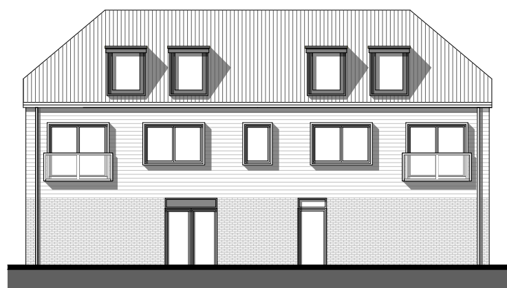
Proposed Rear Elevation 1:200
