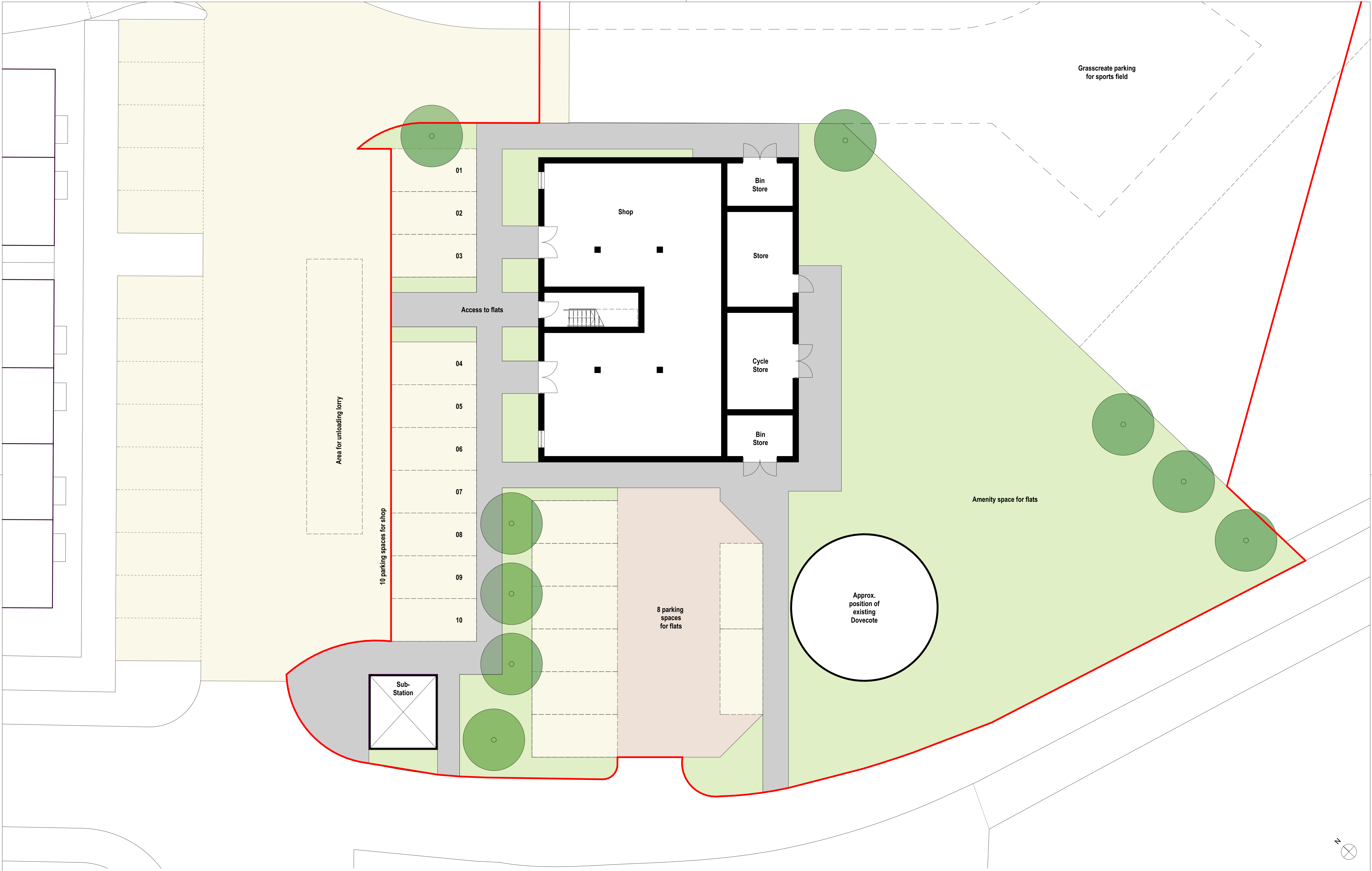
Block Plan
