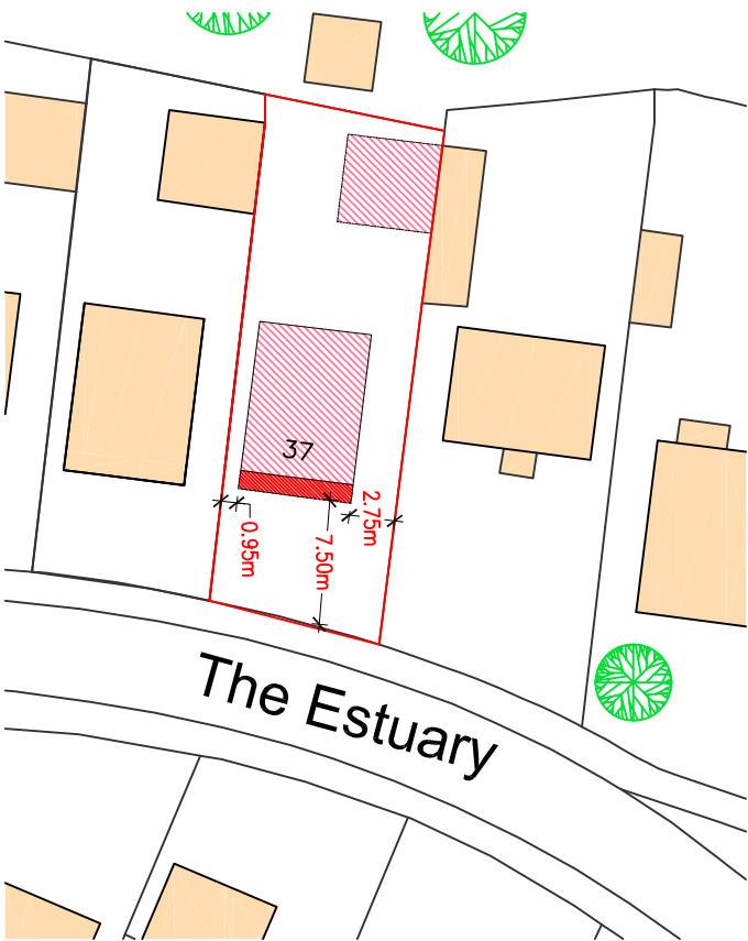
Block Plan - Proposed 0m 5m 10m 15m 20m 1:500 Scale bar
