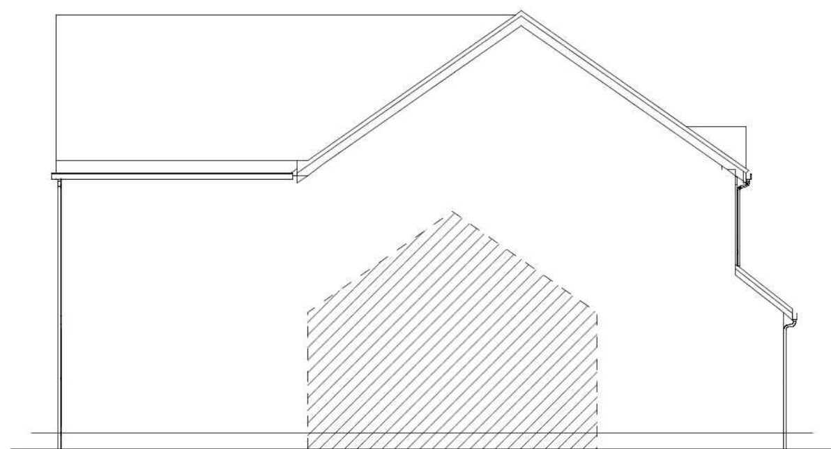
A :: Proposed East Elevation 04 scale: 1:100
