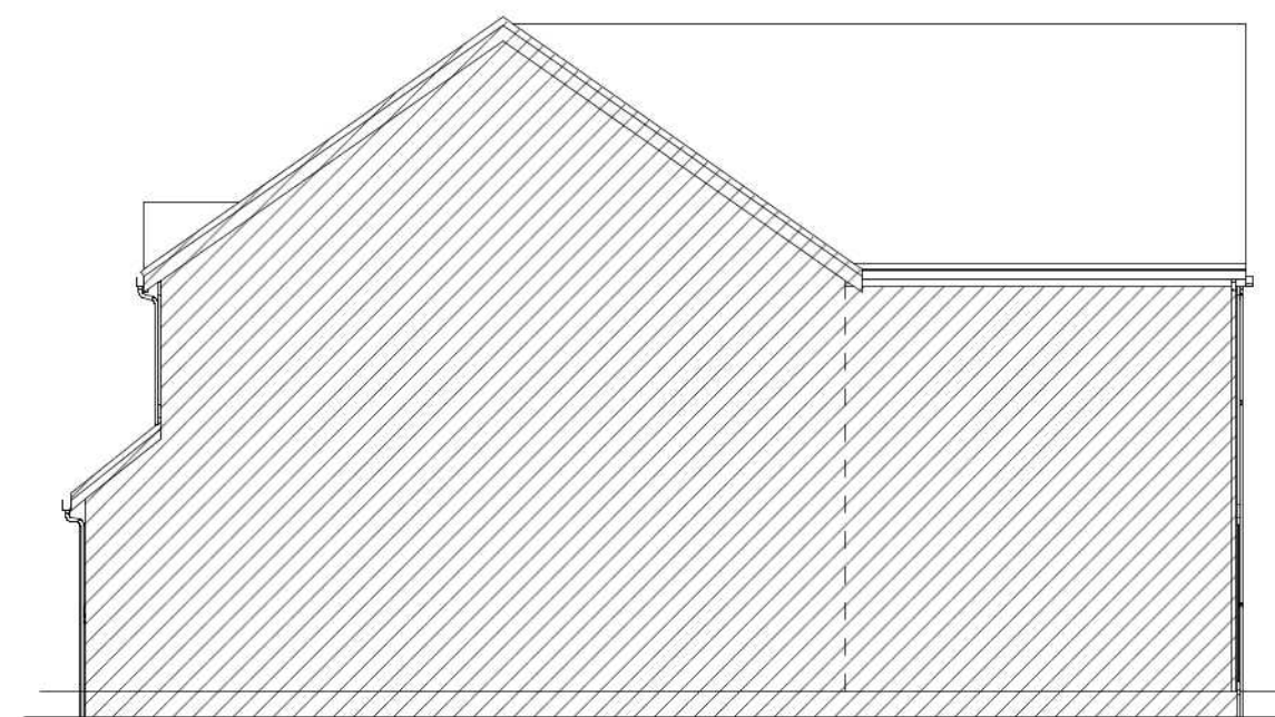
A :: Proposed West Elevation 04 scale: 1:100
