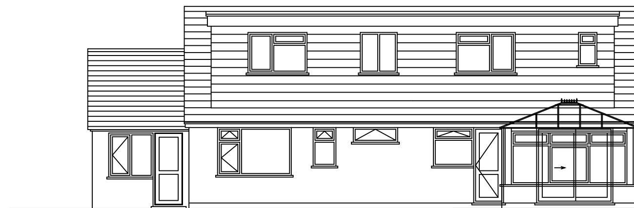
Proposed Rear/NE Elevation
