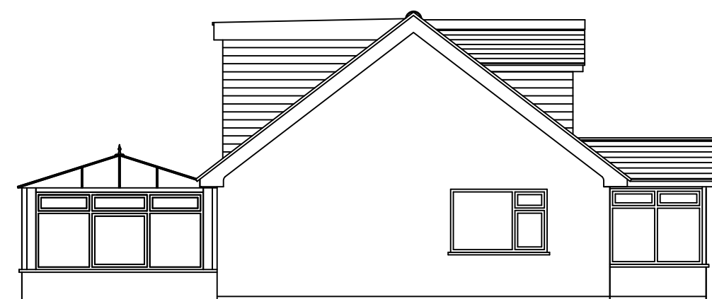
Proposed Side/NW Elevation
