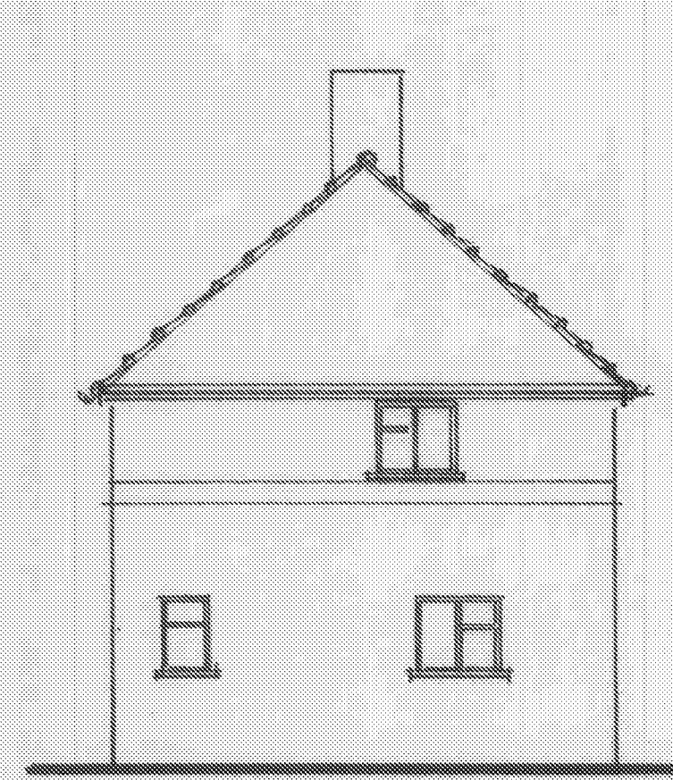
EXISTING SIDE ELEVATION (WEST)
