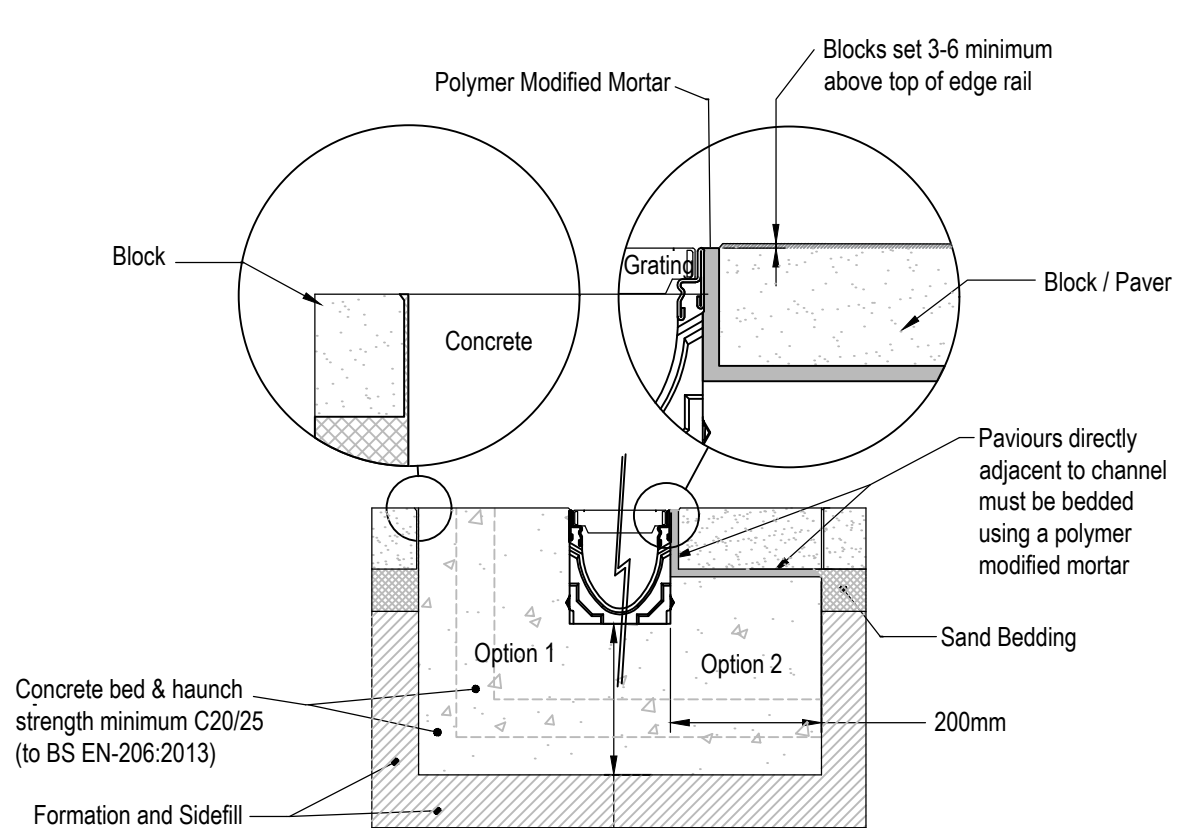
ACO MULTIDRAIN BLOCK PAVEMENT (OPTION 1 & 2) Scale 1:10 @ A1
