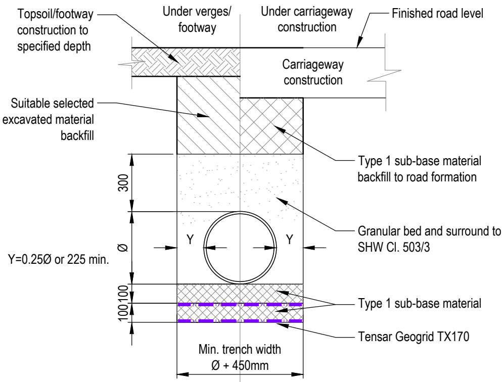
PIPE BEDDING - TYPE S GRANULAR SURROUND WITH GEOGRID Scale 1:20 @ A1
