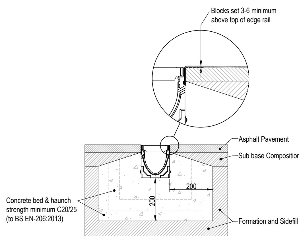
ACO MULTIDRAIN ASPHALT PAVEMENT Scale 1:10 @ A1
