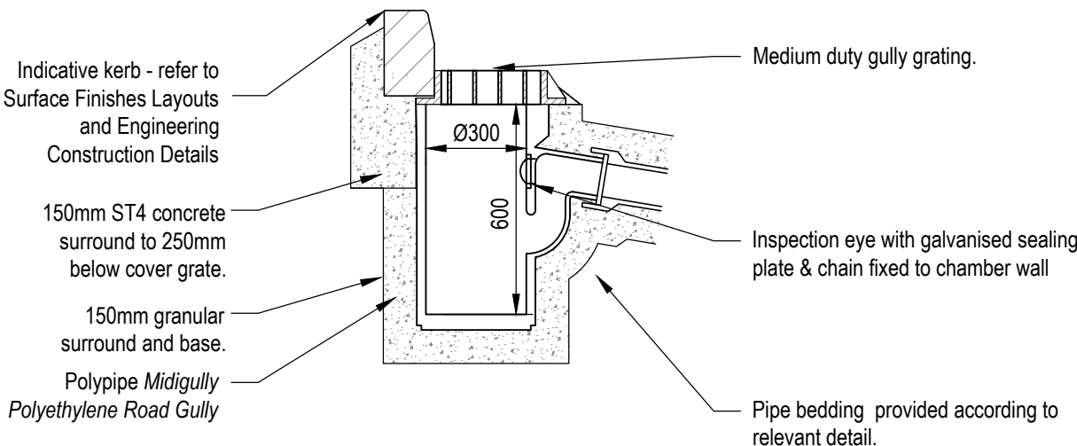
DRIVE GULLY DETAIL (POLYPIPE MIDIGULLY) Scale 1:20 @ A1
