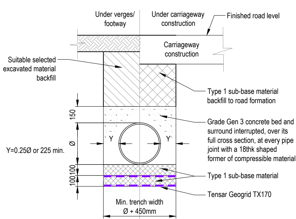
PIPE BEDDING - TYPE Z CONCRETE SURROUND WITH GEOGRID Scale 1:20 @ A1
