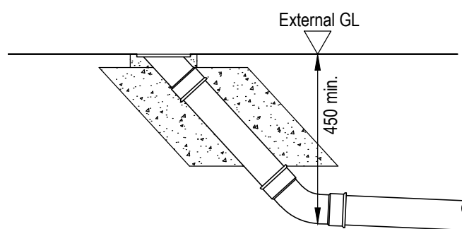
RODDING EYE Scale 1:20 @ A1
