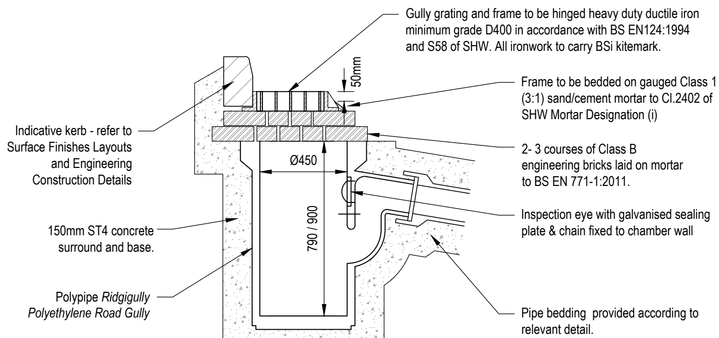
ROAD GULLY DETAIL (POLYPIPE RIDGULLY) Scale 1:20 @ A1
