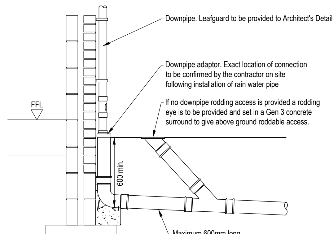
RAINWATER PIPE Scale 1:20 @ A1
