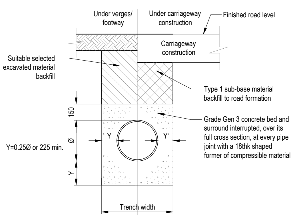
PIPE BEDDING - TYPE Z CONCRETE SURROUND Scale 1:20 @ A1
