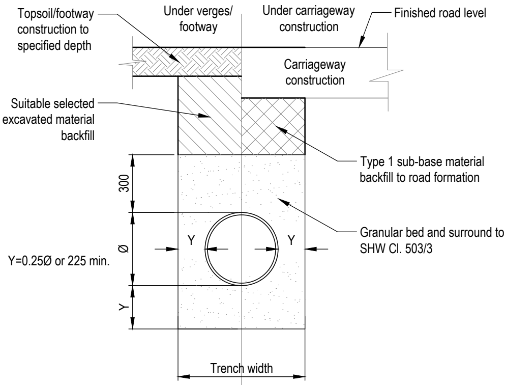
PIPE BEDDING - TYPE S GRANULAR SURROUND Scale 1:20 @ A1
