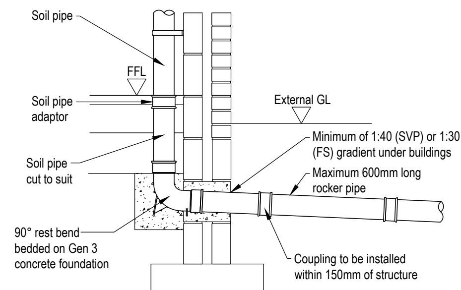
SOIL VENT PIPE Scale 1:20 @ A1
