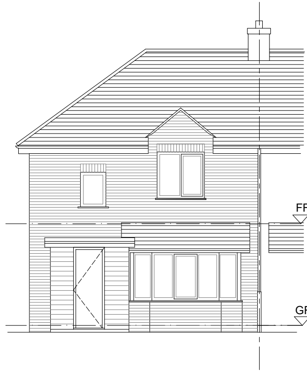
Proposed South Elevation
