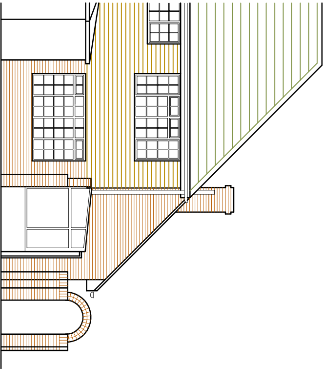
PART EXISTING REAR (EAST) ELEVATION
