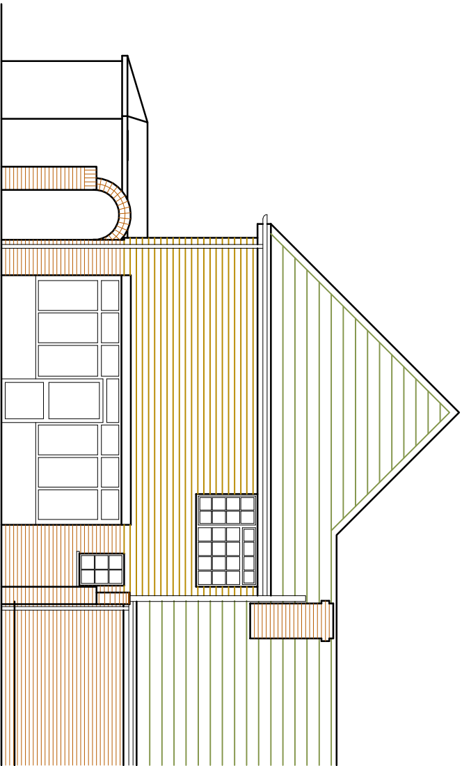
PART EXISTING SIDE (NORTH) ELEVATION
