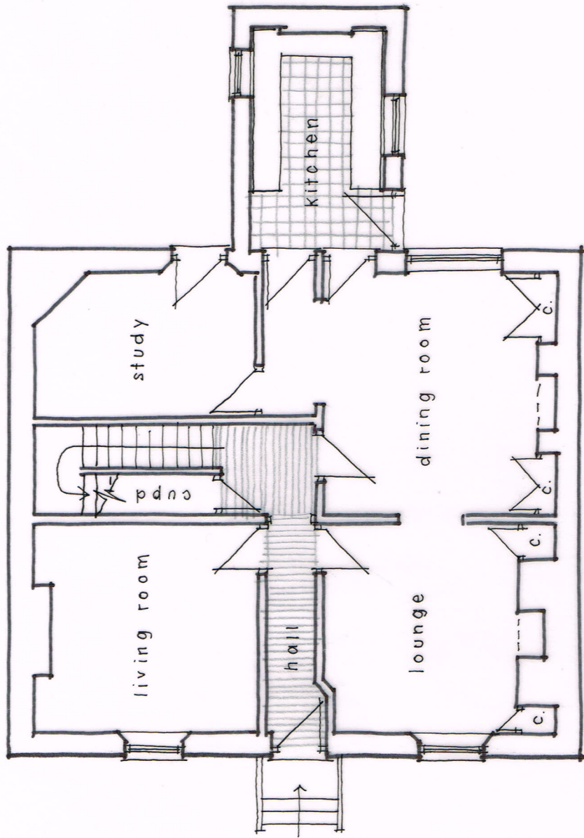
GROUND FLOOR PLAN 1:100 @ A3 1:50 @ A1
