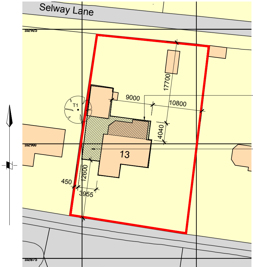
Proposed Site / block plan 1:500 @ A3
