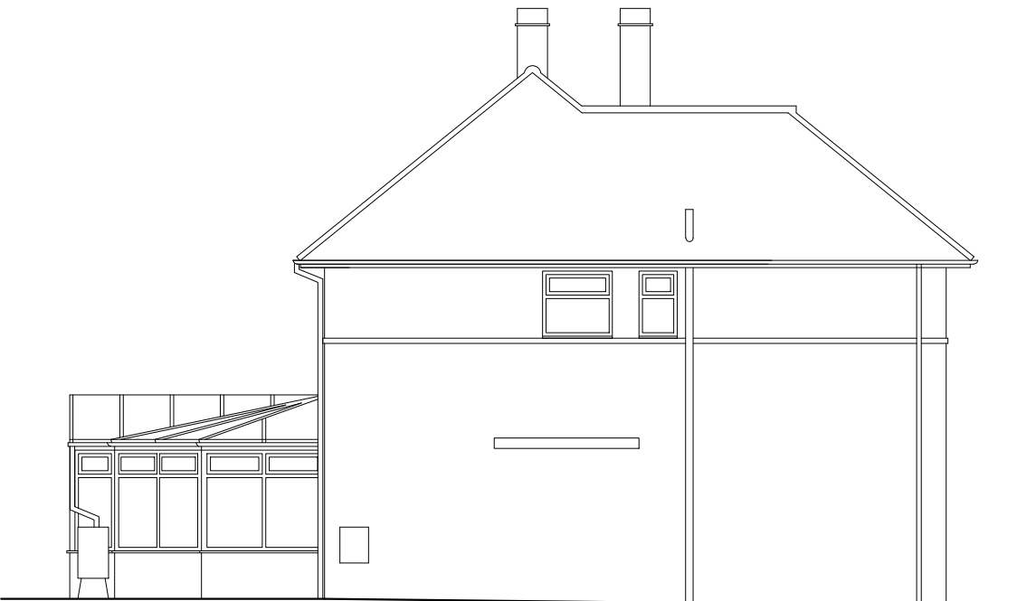
Ex. West Elevation (side) 1:100 @ A3
