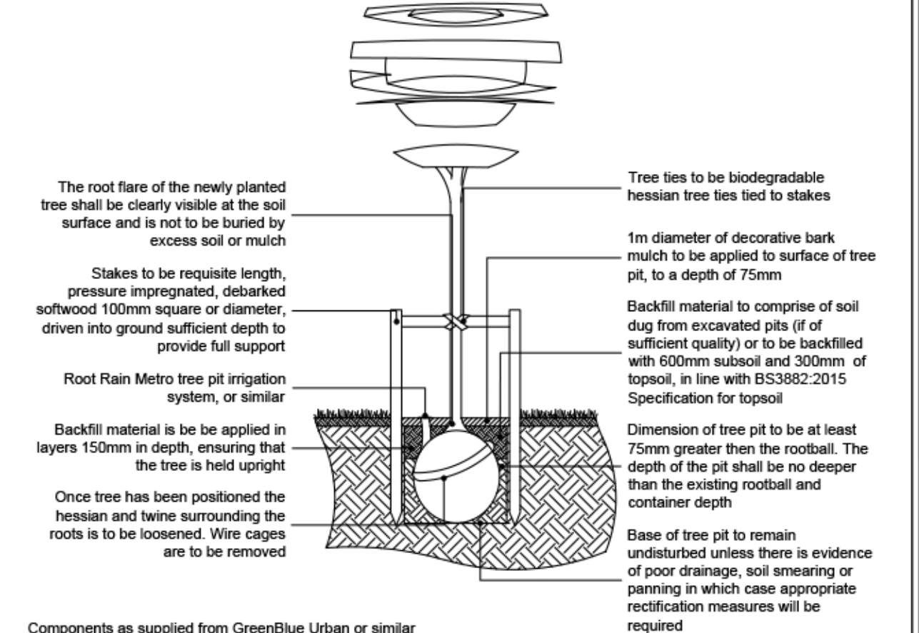
Tree Pit Detail: Soft Landscape
