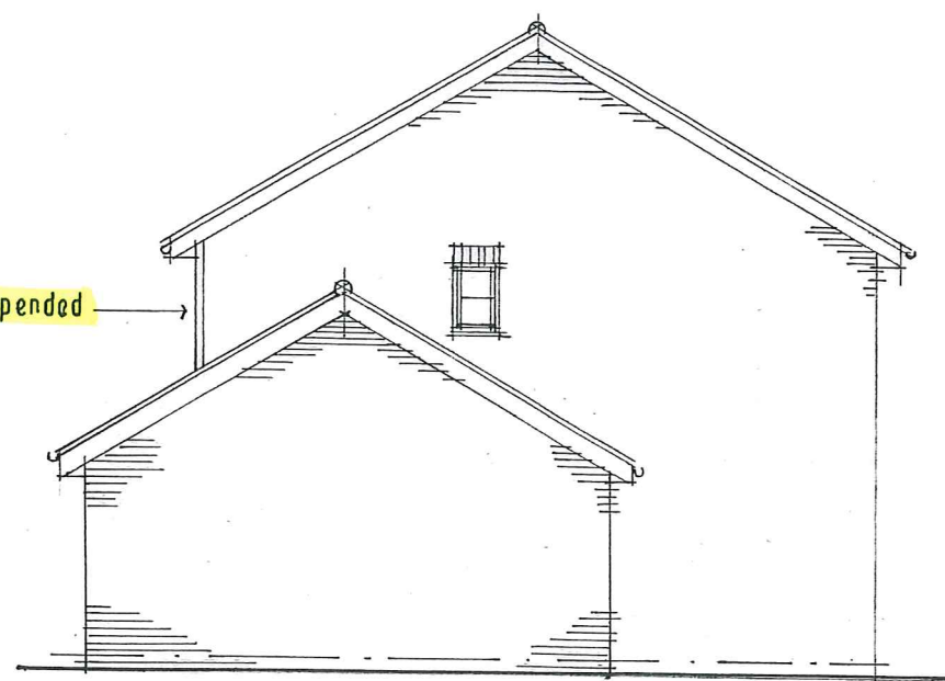
EAST 1/100
