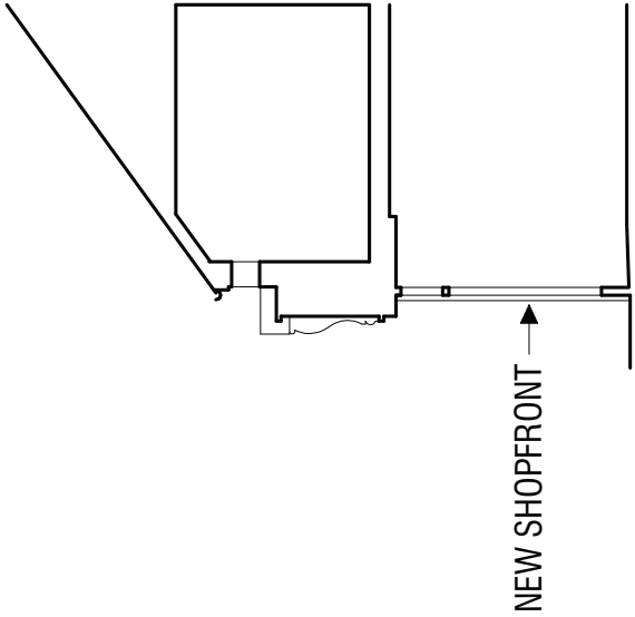
Section at shopfront
