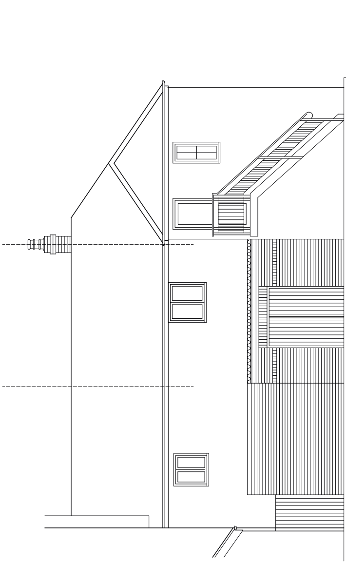
Rear Elevation As Proposed (existing external canopy either renovated or removed)
